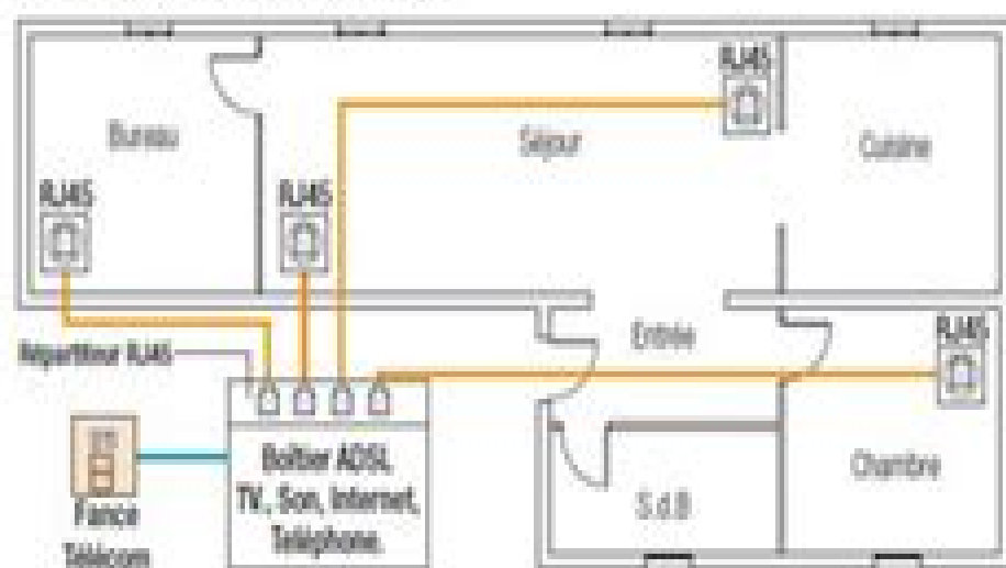
Installation VDI
