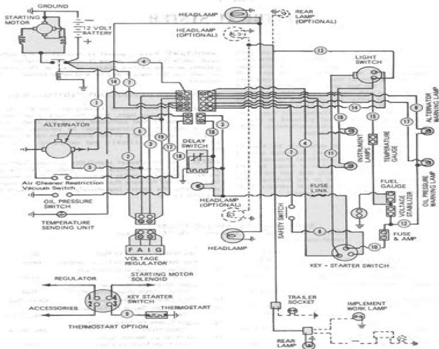
Figure 1 Electrical System Schematic
