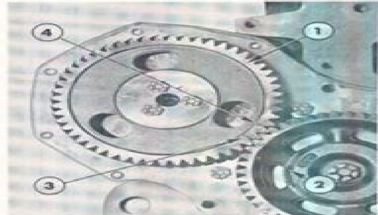
Figure 9 Distributor Type Fuel Injection Pump Drive Gear to Camshaft Drive Gear Timing
