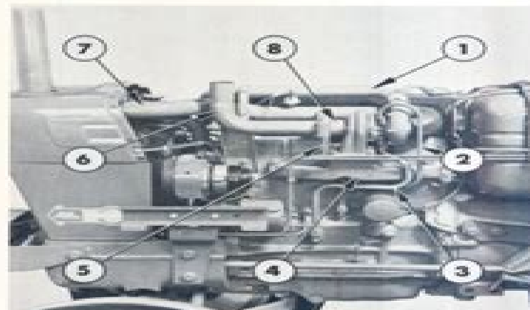
Ford 7600 Turbocharger Component Identification – Left Side
