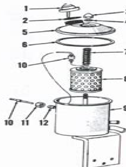
Fig. 6—Exploded view of power steering system reservoir used on 8000 and 9000 models and early 8500 and 9500 models. Oil level switch (10) is connected to warning light on instrument panel. Filter element (8) and oil in reservoir should be renewed after each 500 hours of use.
