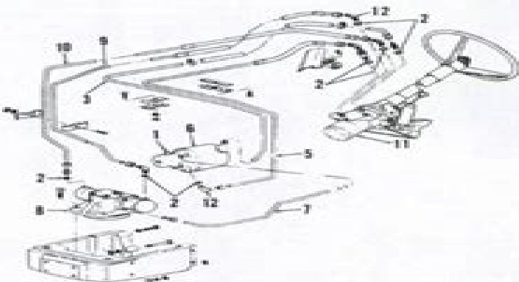
Fig. 4—View showing hydrostatic power steering system used on 8000 and 9000 models and early 8500 and 9500 models. Note that tube (8) from left and of steering motor (8) is connected to lower port on front side of Hydramotor steering unit (11) and is connected by long fitting to offset connecting tube. Pressure tube (5) from pump is connected to left side port of Hydramotor unit by elbow (12); elbow (13) is fitted in rear port of Hydramotor unit and connects to return tube (7) to reservoir. Refer to Fig. 5 for later systems.
