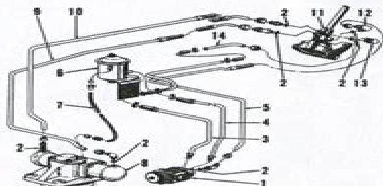
Fig. 4—View showing hydrostatic power steering system used on 8000 and 9000 models and early 8500 and 9500 models. Note that tube (8) from left and of steering motor (8) is connected to lower port on front side of Hydramotor steering unit (11) and is connected by long fitting to offset connecting tube. Pressure tube (5) from pump is connected to left side port of Hydramotor unit by elbow (12); elbow (13) is fitted in rear port of Hydramotor unit and connects to return tube (7) to reservoir. Refer to Fig. 5 for later systems.
