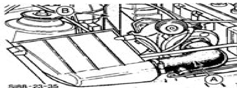
Fig.45. A - Top air hose B - Heat shield
