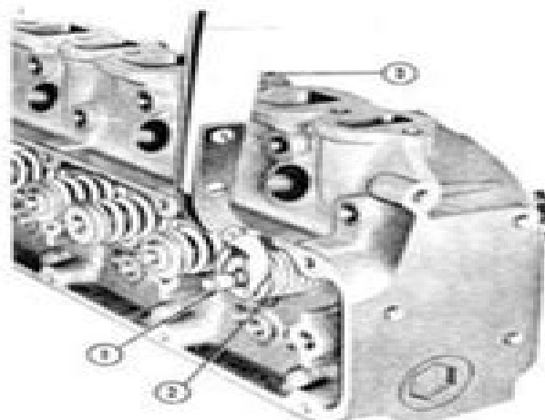
Figure 5 Removing Valves
