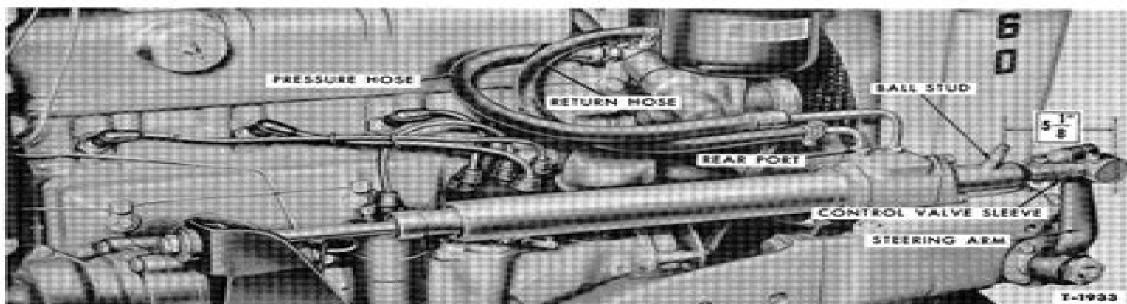
Figure 28—Adjustment of Power Cylinder and Control Valve to Steering Arm
