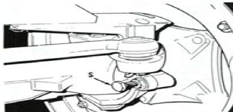
Fig. 7—Steering stop screws (S) should be adjusted to prevent tires from touching any part of tractor when wheels are turned.
