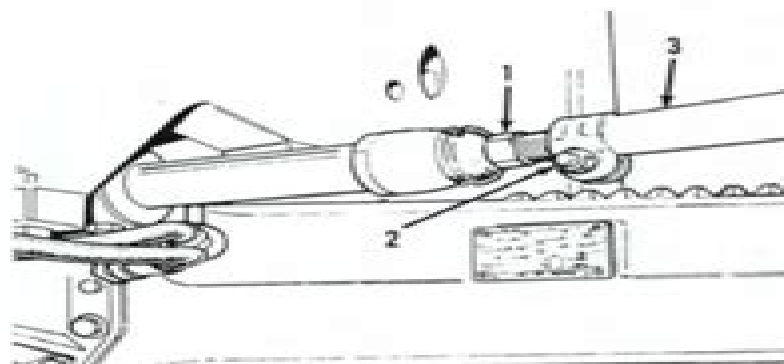
Fig. 6—View of toe-in adjustment points for four-wheel-drive models. Be sure to adjust both sides equally. Refer to text.
