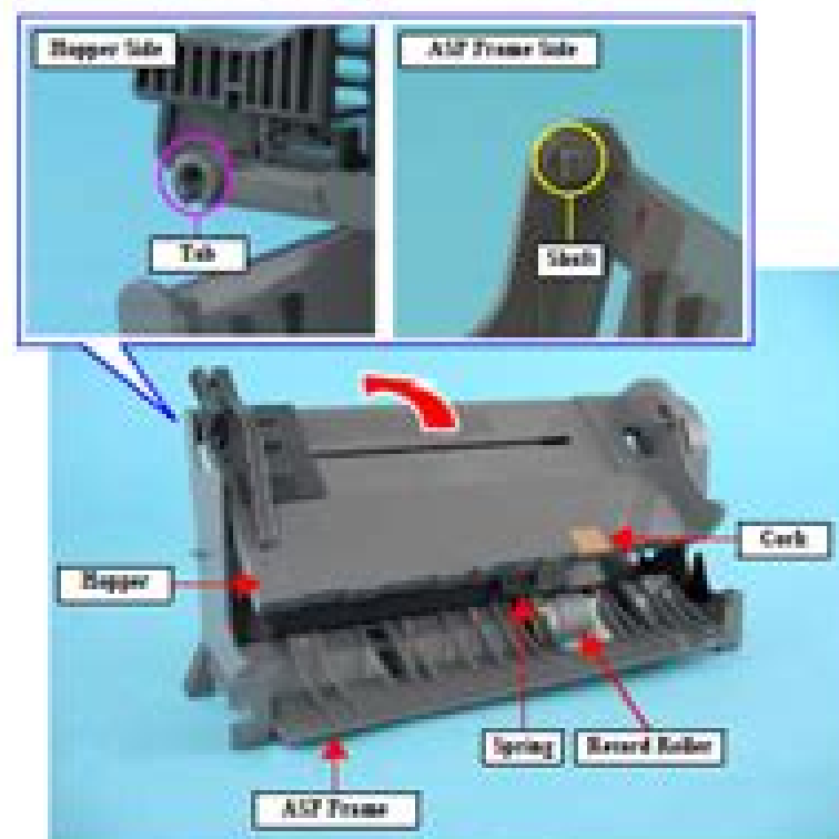
Figure 4-7. Removing Hopper
