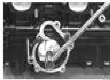
11. Apply sealant to the crankcase cover, then install the oil-injection pump timing driving screw.
