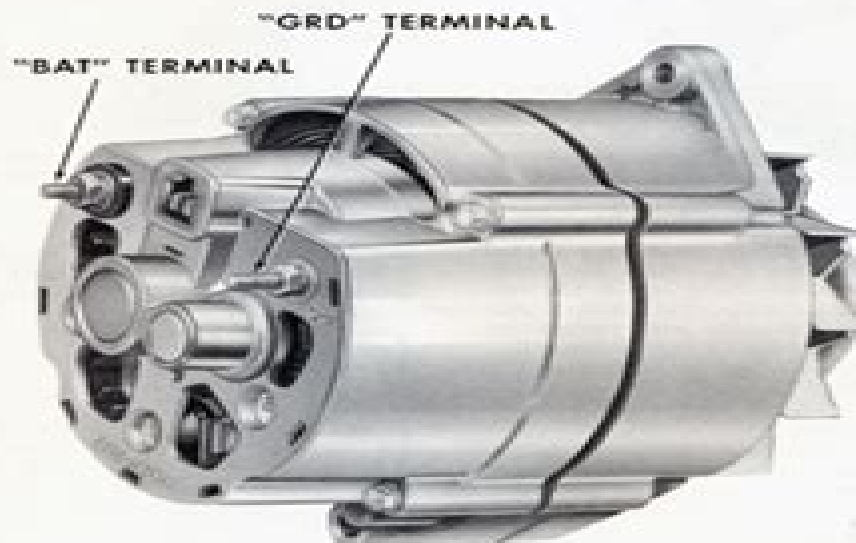
Figure 1—Typical "Delcotron"
