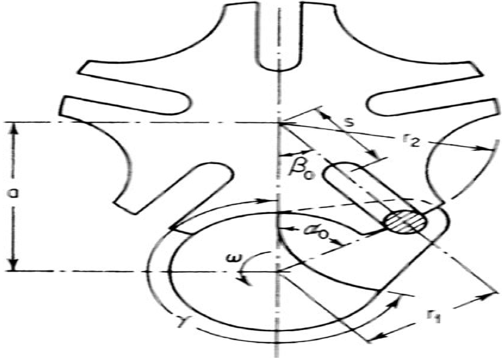
FIG. 3.54 External geneva mechanism in starting position.
