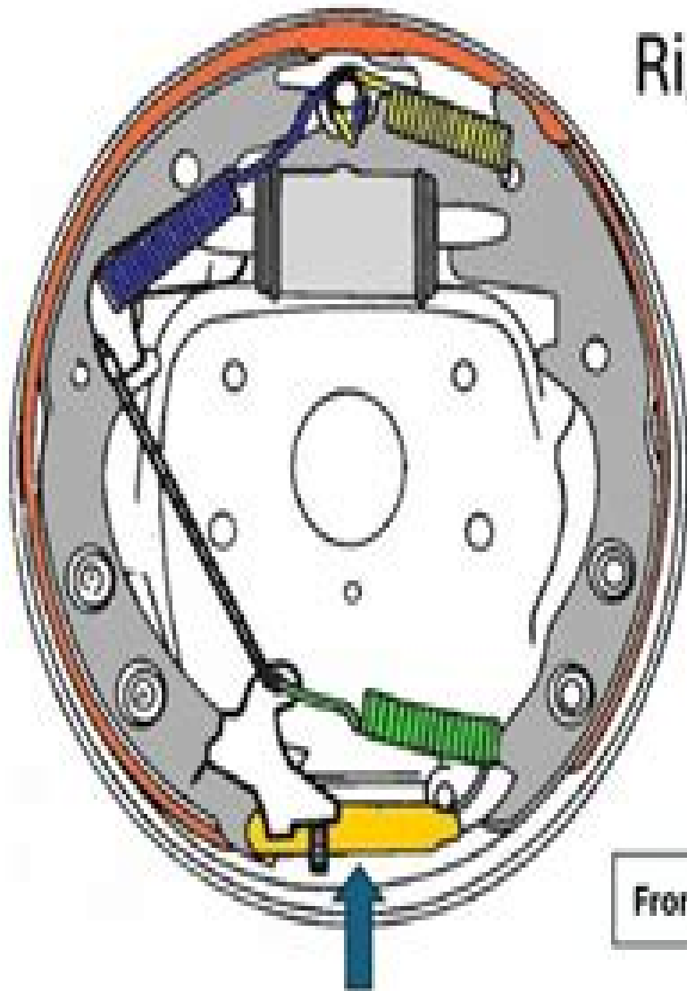
Duo-Servo Drum Brakes Shoes Anchored only at the Top. Free Floating Adjuster At the Bottom
