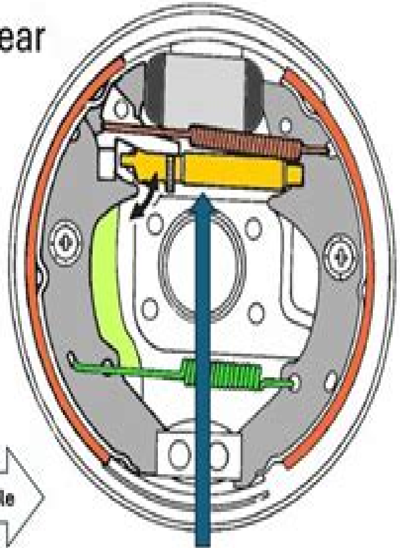
Leading-Trailing Drum Brakes Shoes Anchored at the Bottom. Adjuster Right Under the Wheel Cylinder
