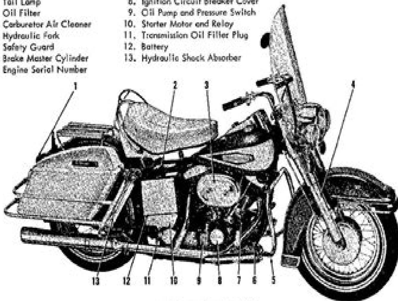
FIGURE 1. RIGHT SIDE VIEW
